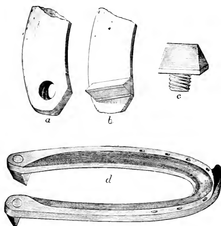
FIG. 131.—WHITE'S PLAN OF ROUGHING SHOES.
